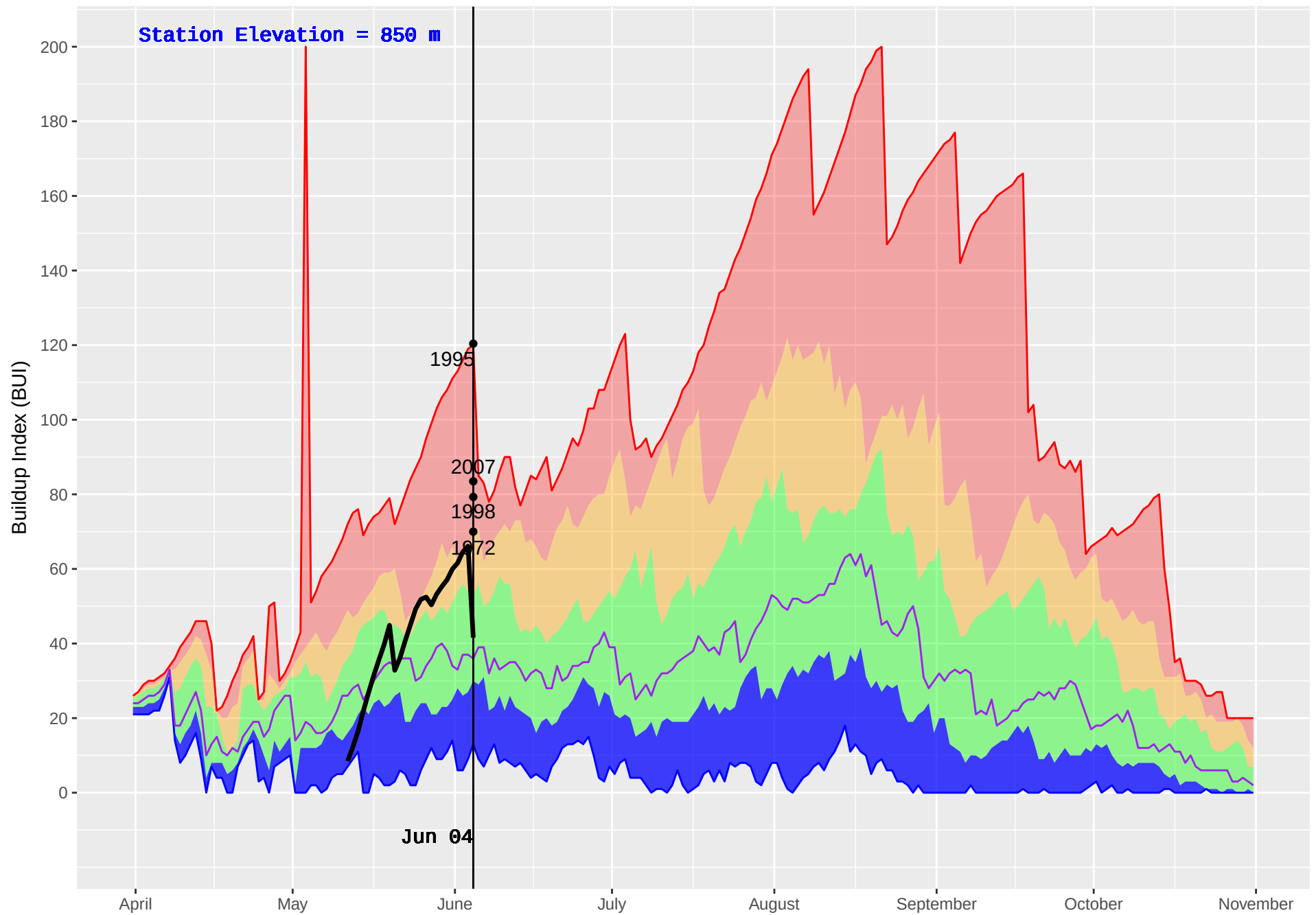
NORTH CHILCO (159) : Historical (1972–2016) and Current (2018) Noon Buildup Index (BUI)
