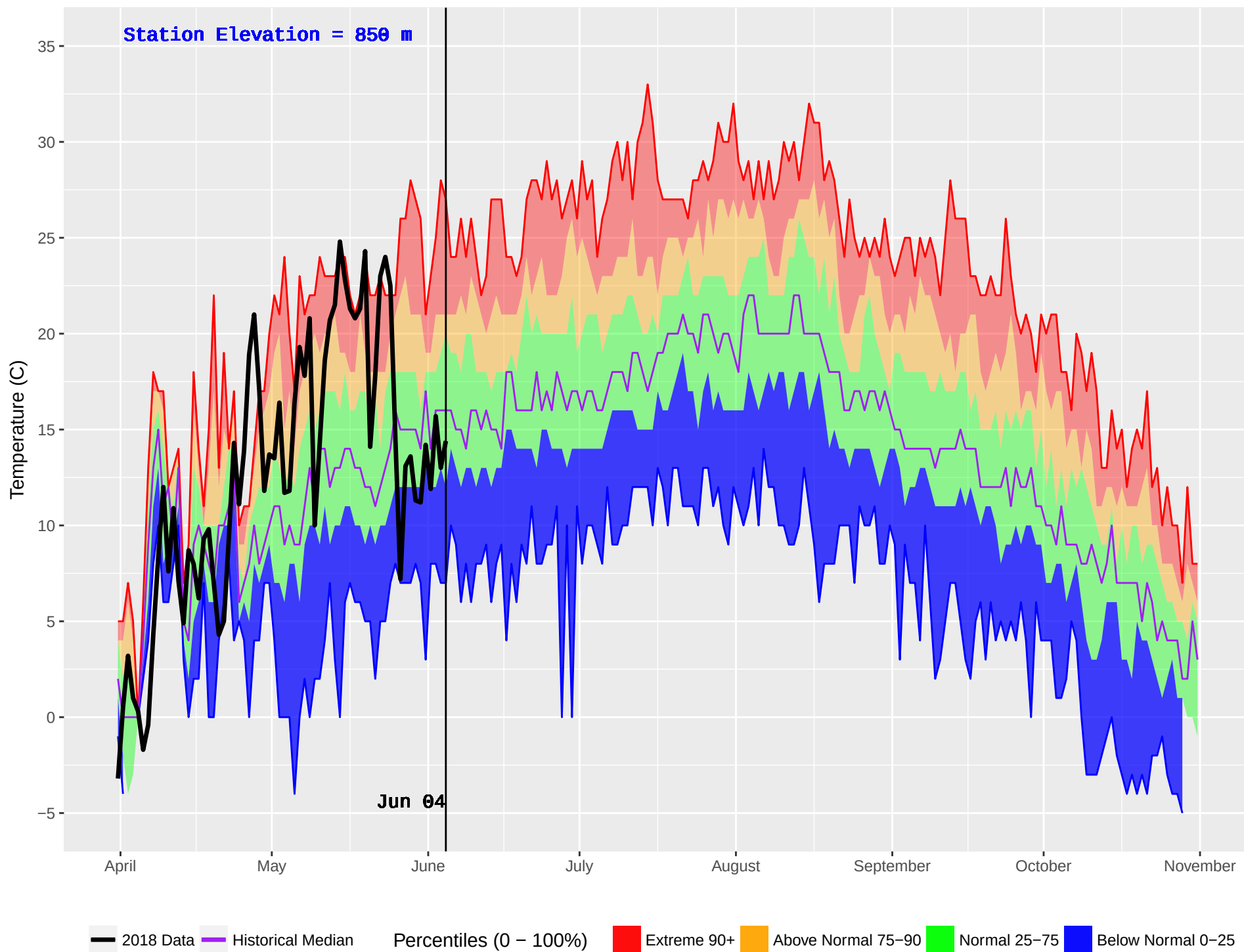
NORTH CHILCO (159) : Historical (1972–2016) and Current (2018) Noon Temperature
