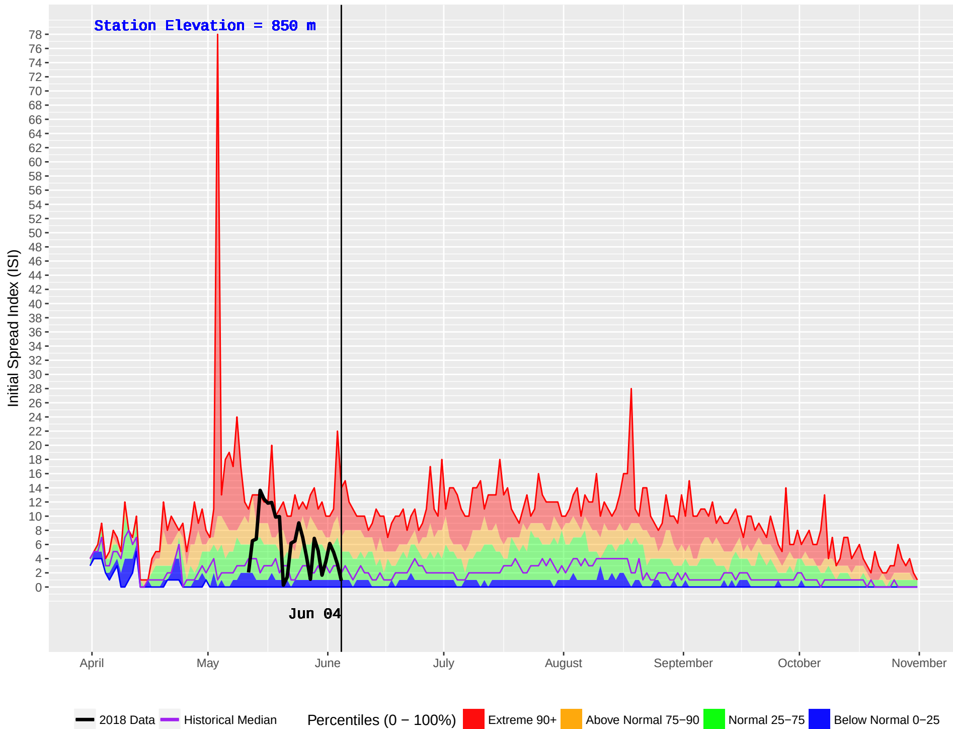
NORTH CHILCO (159) : Historical (1972–2016) and Current (2018) Noon Initial Spread Index (ISI)
